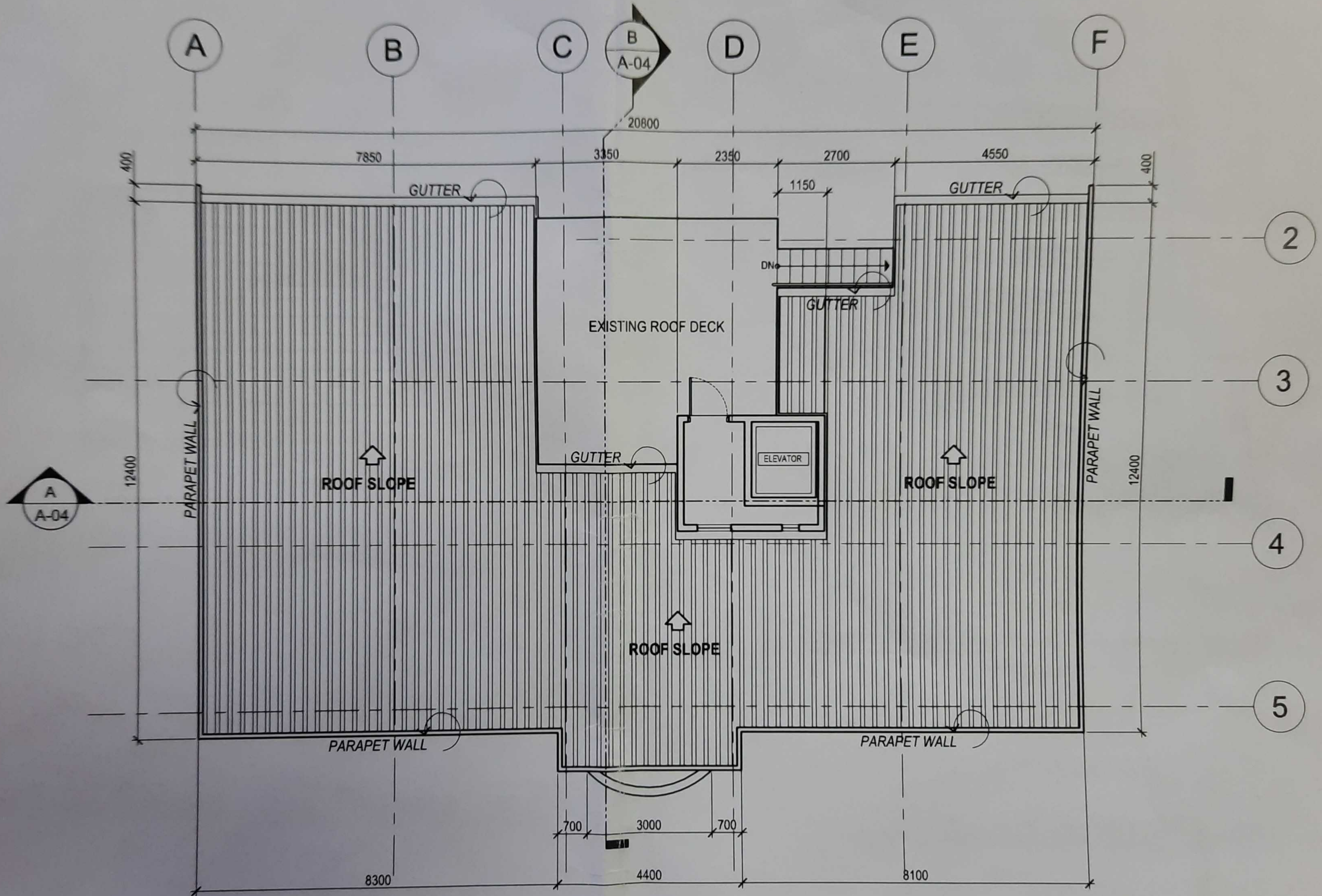
B A-02 ROOF DECK SCALE 1 : 100 MTS.
